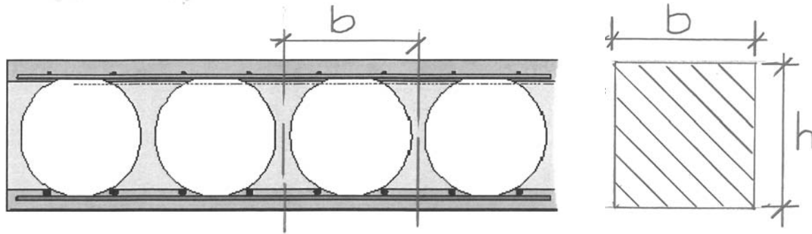
(a) Elements of a voided slab
